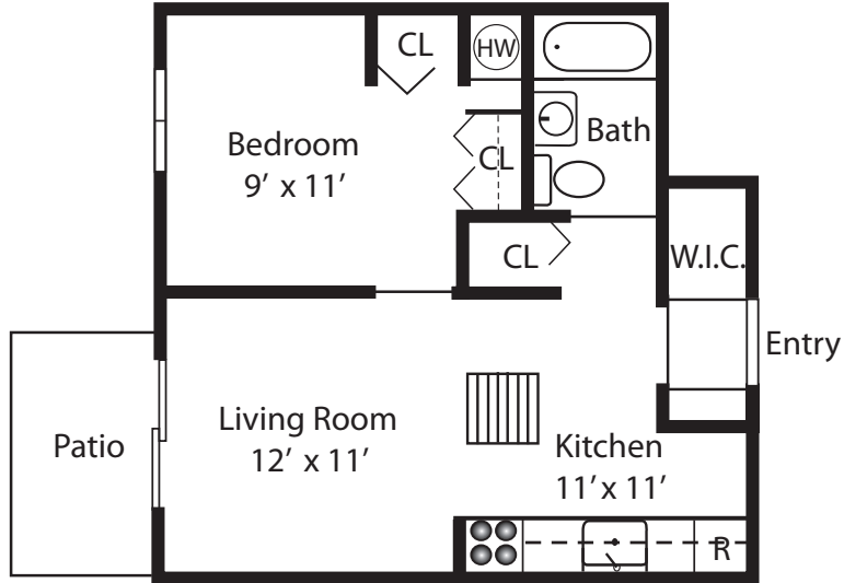
Regular Unit - First Floor One Bedroom - 605 Sq. Ft.
